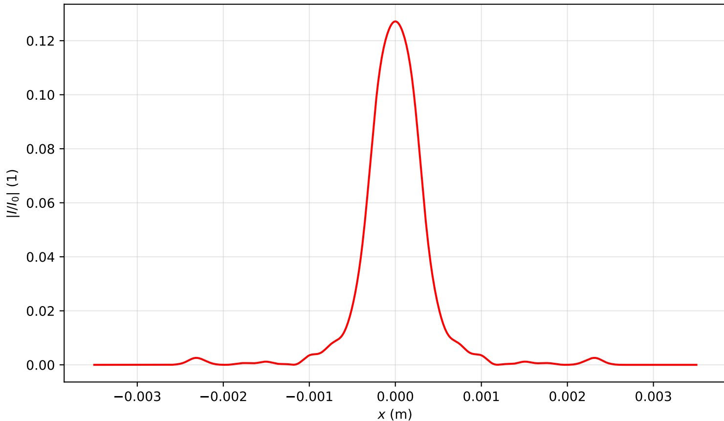
Intensity profile I(x, y = 0, z = 3.503)/I_0 , P_{in}=6.0P_{cr} , artificial time
